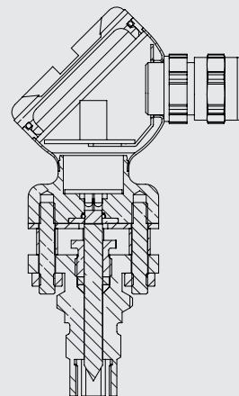
Mounting thread without cooling element
