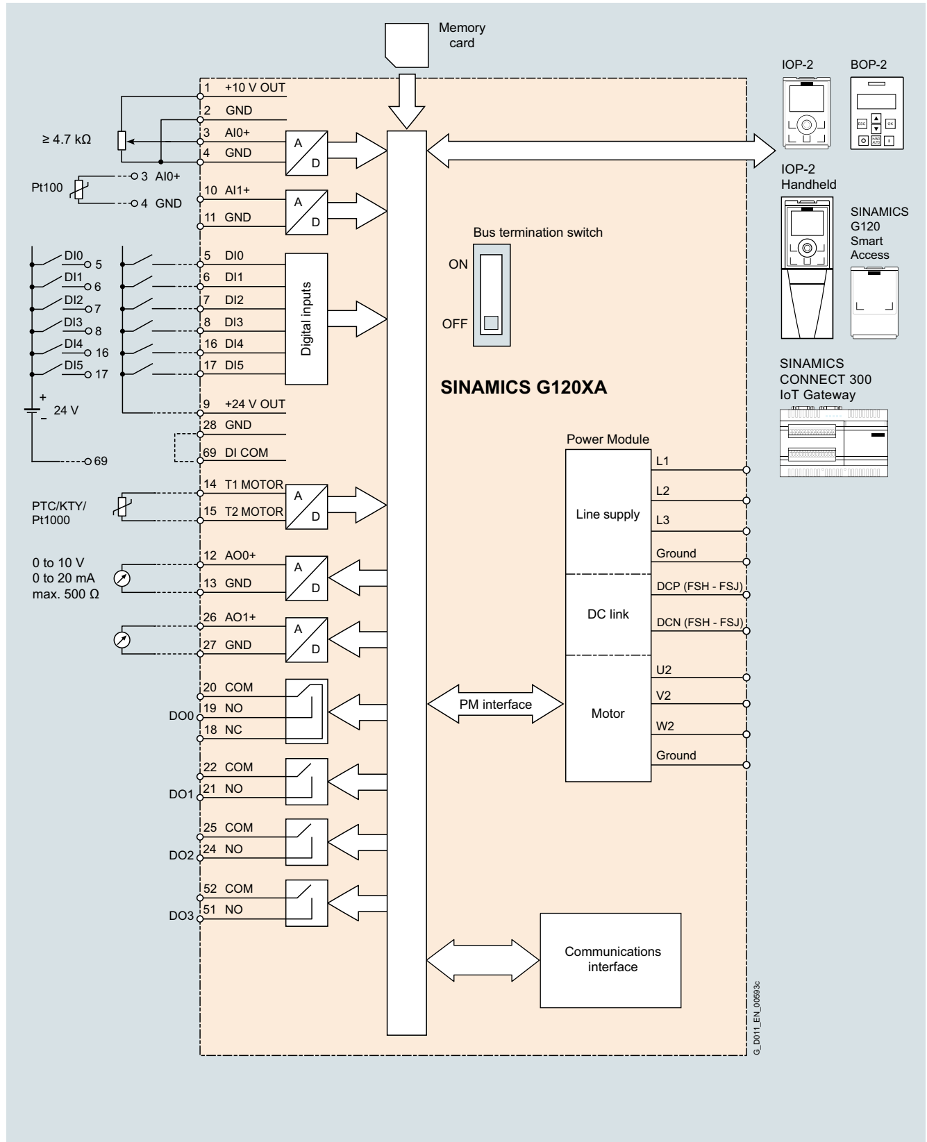
SINAMICS G120XA connection diagram
