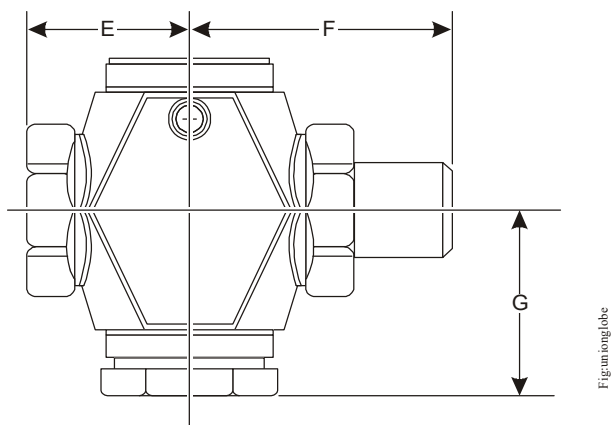
Figure 3: Two-Way N.O./PDTC and Two-Way N.C./PDTO Union Globe Valve Dimensions (See Table 3.)
