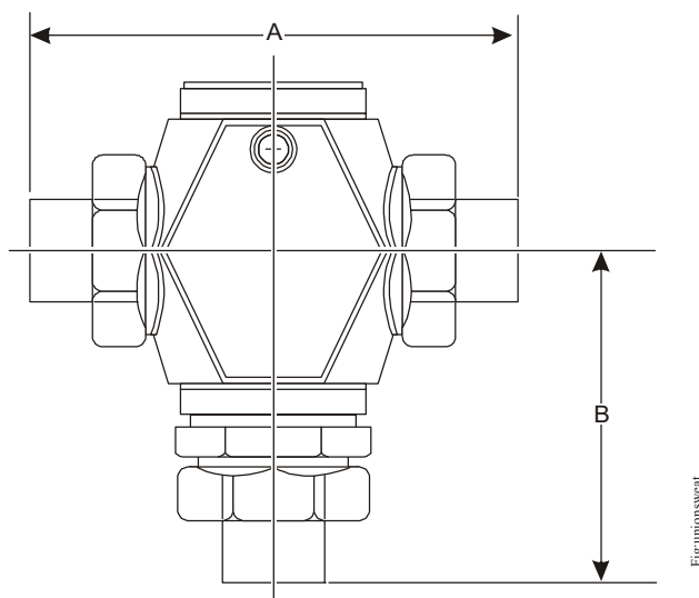
Figure 5: Two-Way N.O./PDTC, Two-Way N.C./PDTO, and Three-Way Mixing Union Sweat Valve Dimensions (See Table 5.)
