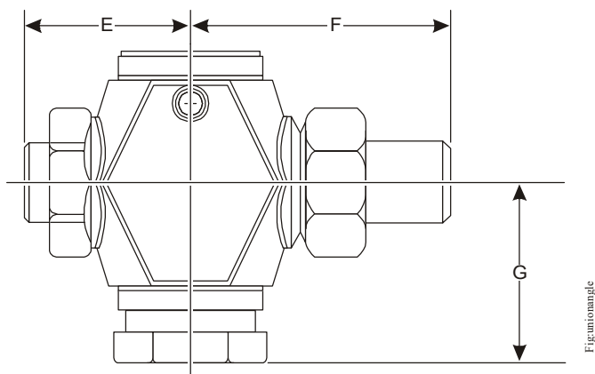
Figure 4: Two-Way N.O./PDTC Union Angle Valve Dimensions (See Table 4.)
