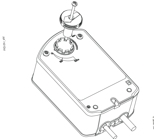
Figure 14: Installing the fixed pointer
