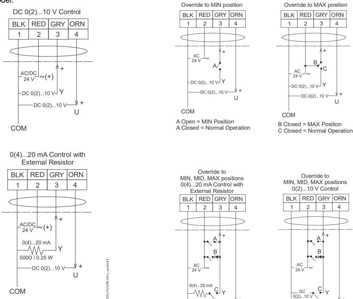
Figure 19: Control wiring diagrams
