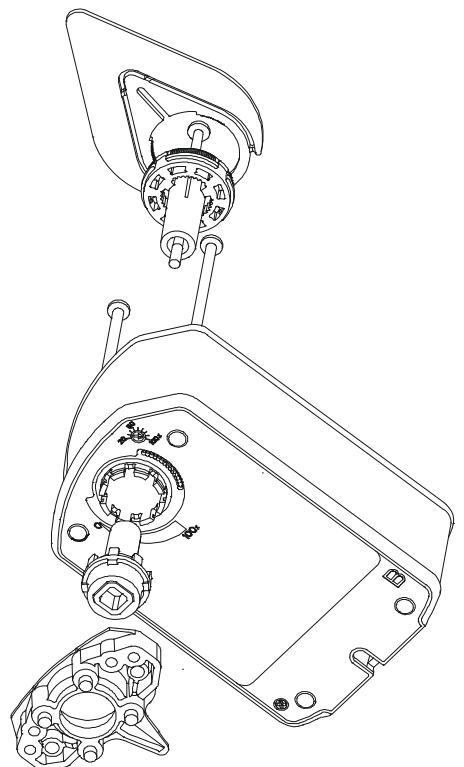
Figure 11: Removing the Linkage
