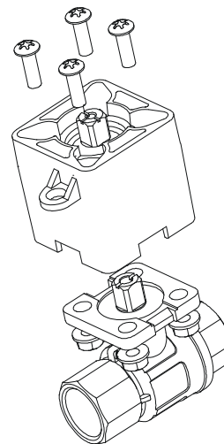
Figure 18: Installing the Barrier
