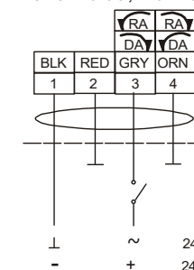
On/Off Control, Two Wire
