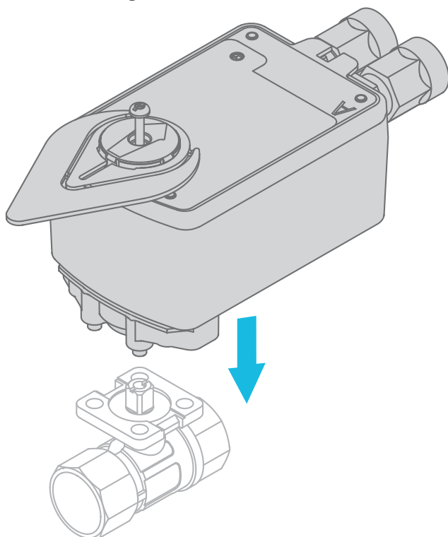
Figure 9: Mounting the actuator
