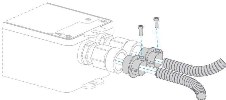
Figure 21: Adding flexible metal conduit
