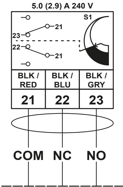
Figure 20: Optional auxiliary switch wiring diagram
