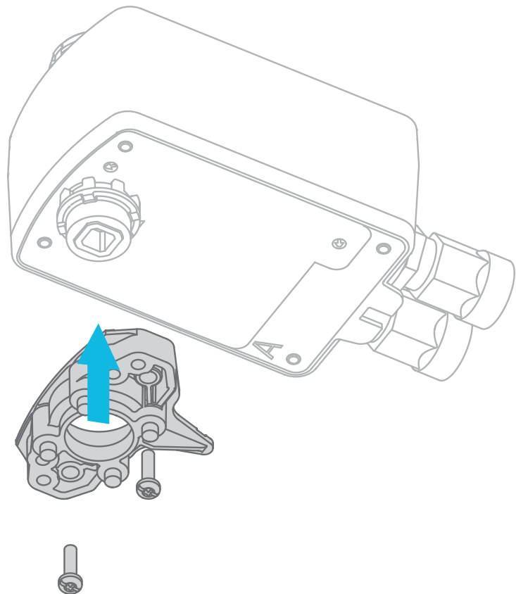
Figure 13: Installing the linkage
