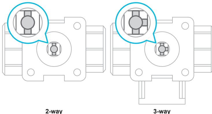
Figure 10: Positioning the valve stem
