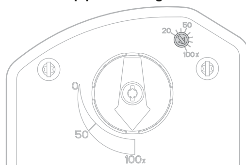
Figure 22: Switch trip point settings
