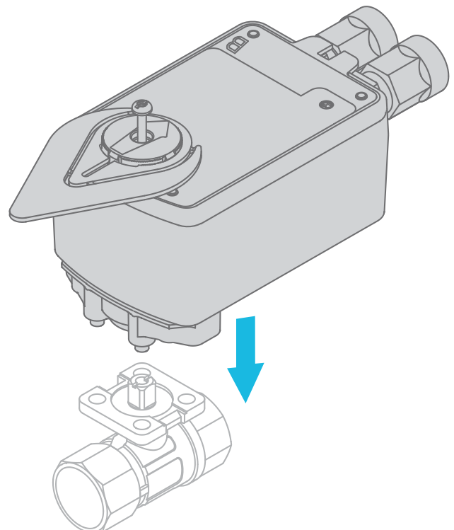
Figure 15: Mounting the actuator
