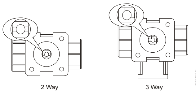
Figure 4: Positioning the valve stem
