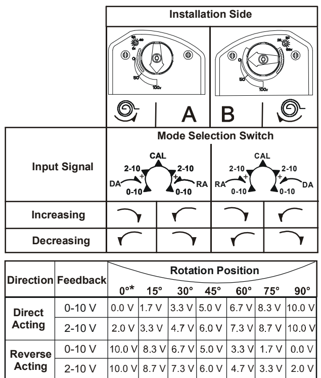
Figure 24: Control response
