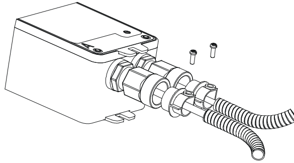
Figure 22: Adding flexible metal conduit
