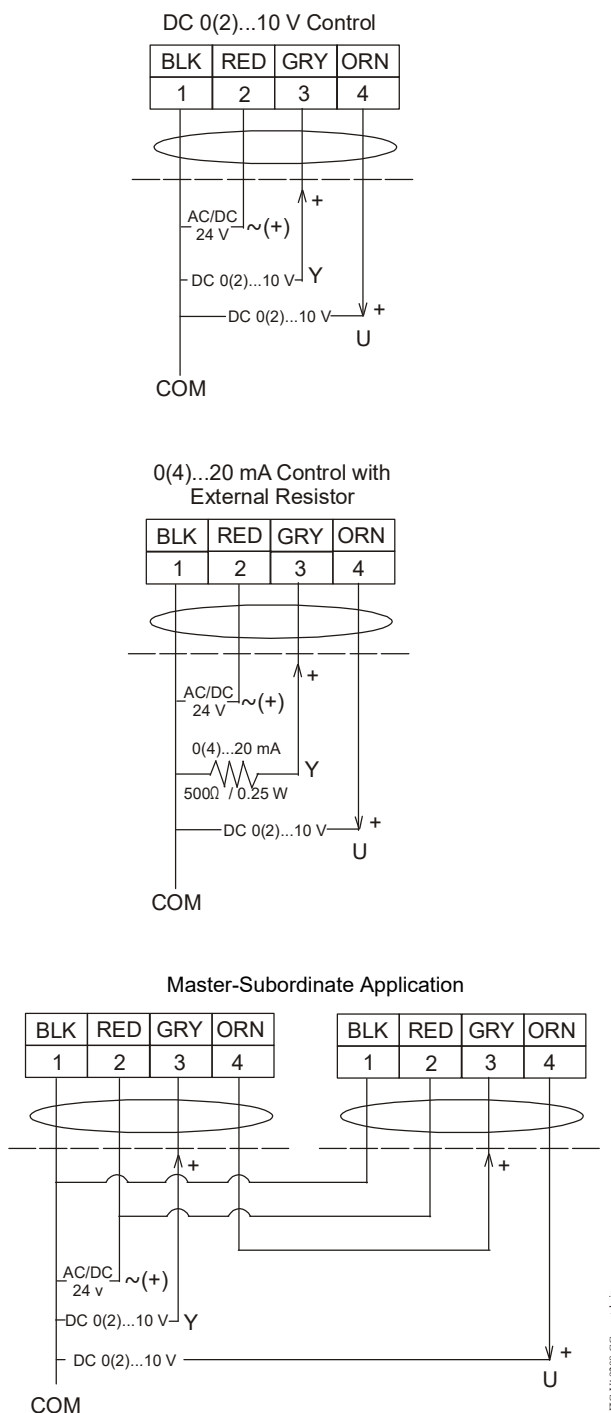
Figure 19: Control wiring diagrams
