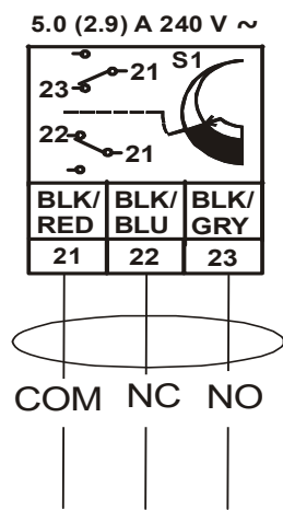
Figure 21: Auxiliary switch wiring diagram
