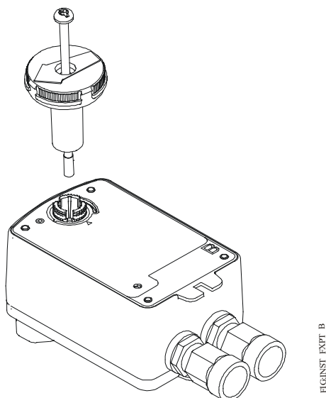
Figure 14: Installing the fixed pointer
