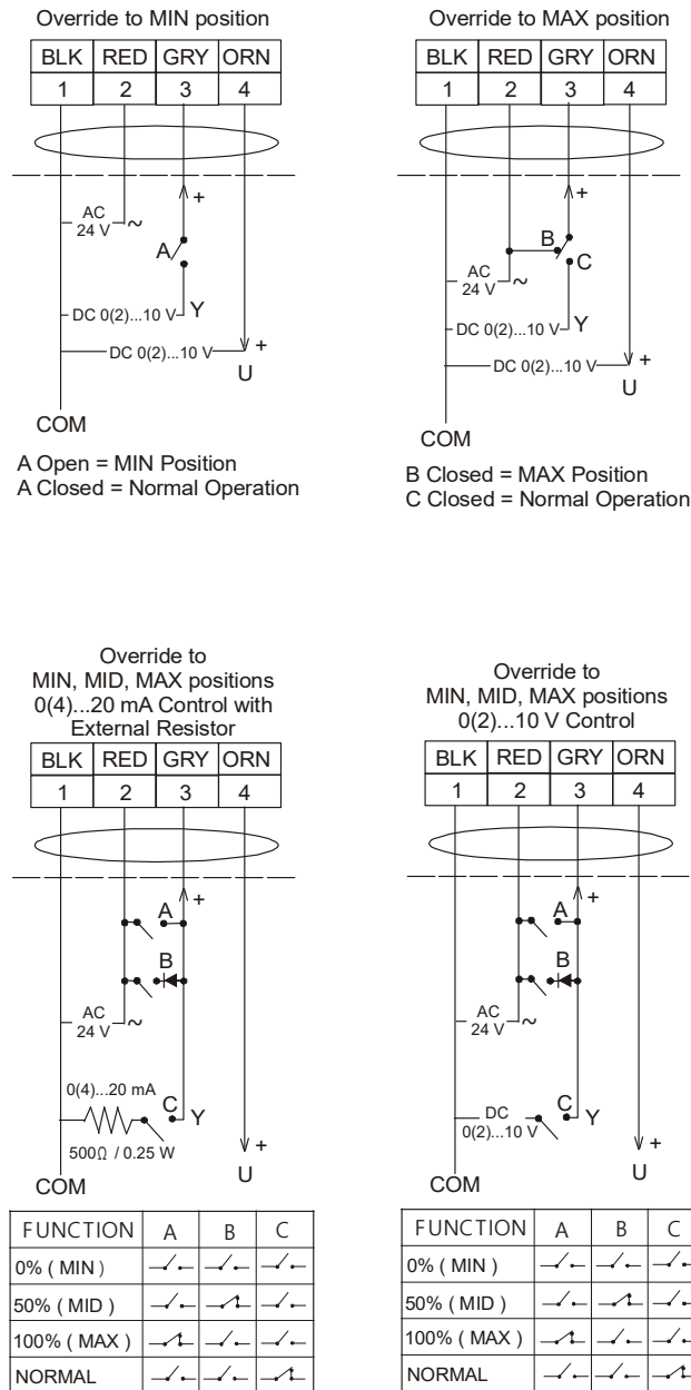
Figure 20: Control wiring diagrams (overrides)
