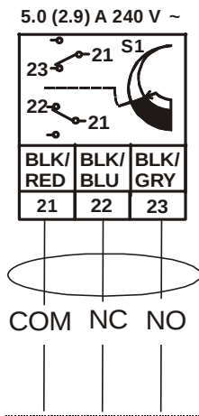
Figure 20: Optional Auxiliary Switch Wiring
