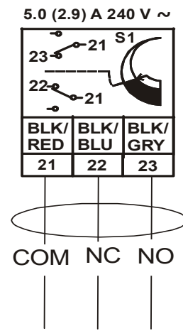
Figure 20: Auxiliary switch wiring diagram
