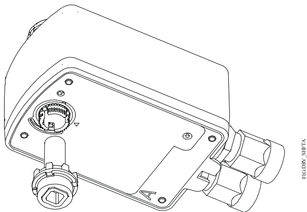
Figure 12: Inserting the drive shaft
