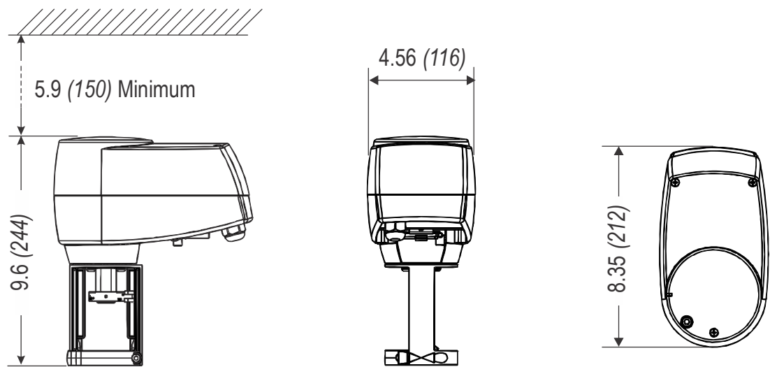
Figure 4: Dimensions, in. (mm)
