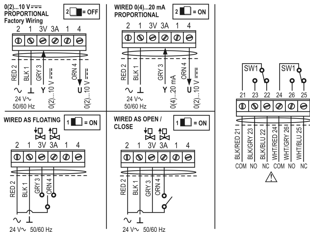
Figure 2: VA78x0-HGx-2 Wiring Diagram
