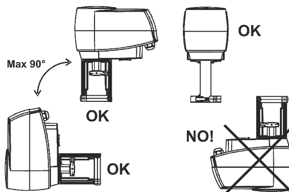
Figure 3: VG7800 Mounting
