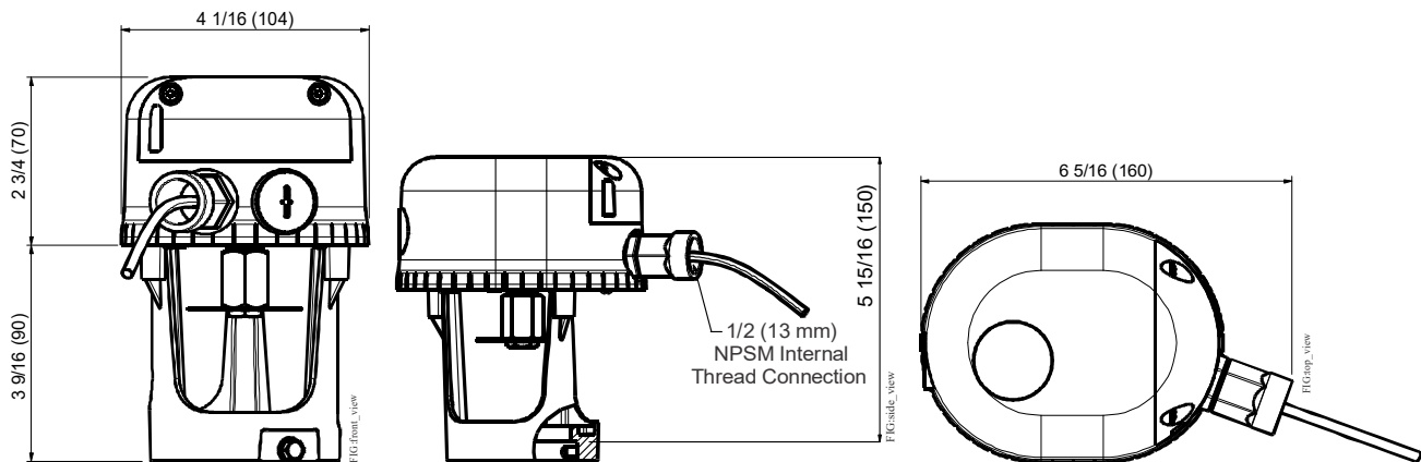
Figure 3: VA-7700 Series actuator dimensions, in. (mm)
