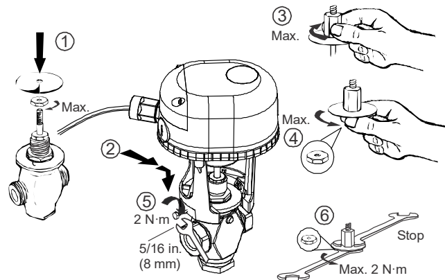
Figure 2: VA-7700 Series actuator installation
