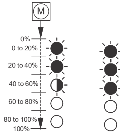
Figure 11: Actuator stem between 40% to 60% of stroke
