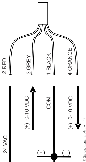
Figure 5: Wiring diagram for VA-7700-GGA-2 proportional model, 24 VAC applications
