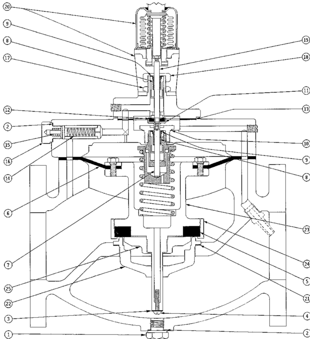
Figure 1: V43 Pressure Actuated Valve Cutaway
