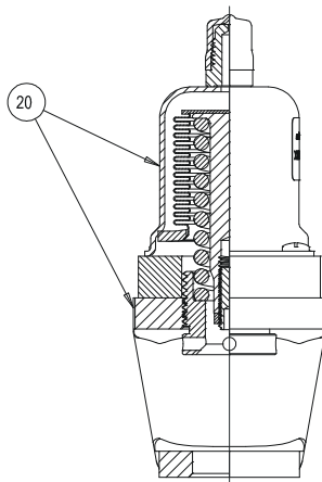
Figure 2: V243 Sensing Element and Yoke
