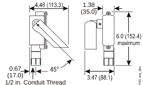
Figure 1: Outdoor Air Sensor Dimensions, in. (mm)
