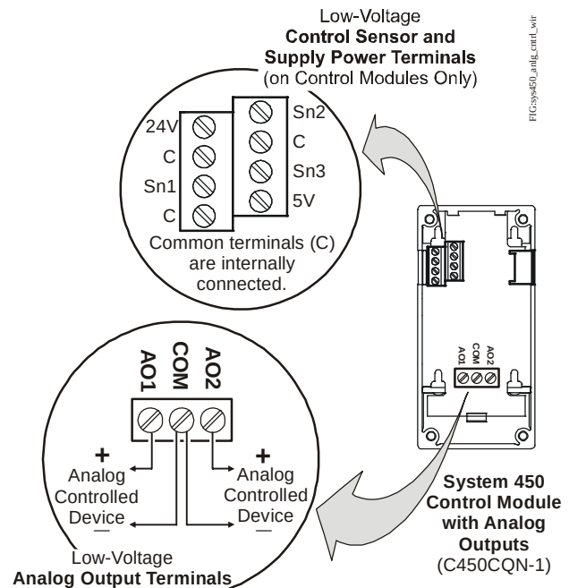
Figure 2: C450CxN-1 Wiring Terminals
