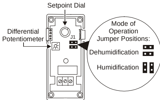
Figure 7: S351 Stage Module Adjustment and Potentiometer Locations
