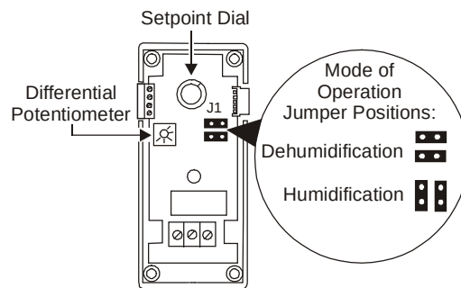
Figure 2: W351 Electronic On/Off Humidity Control; Setpoint and Differential Adjustments; Humidification and Dehumidification Modes
