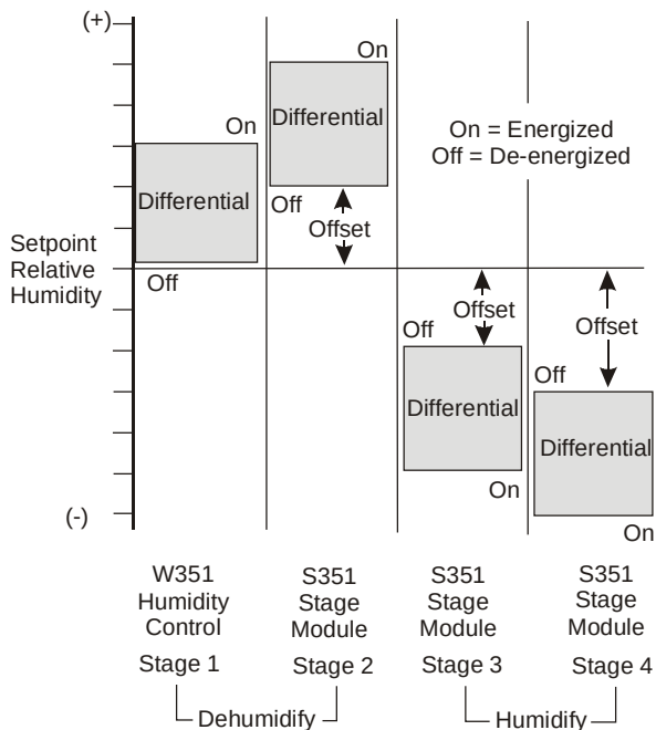
Figure 8: Typical Multistage Humidification/Dehumidification Application
