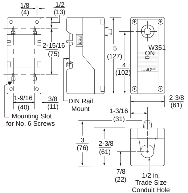
Figure 4: W351 Control Dimensions, in./mm
