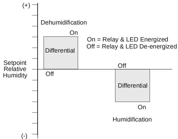
Figure 3: Modes of Operation
