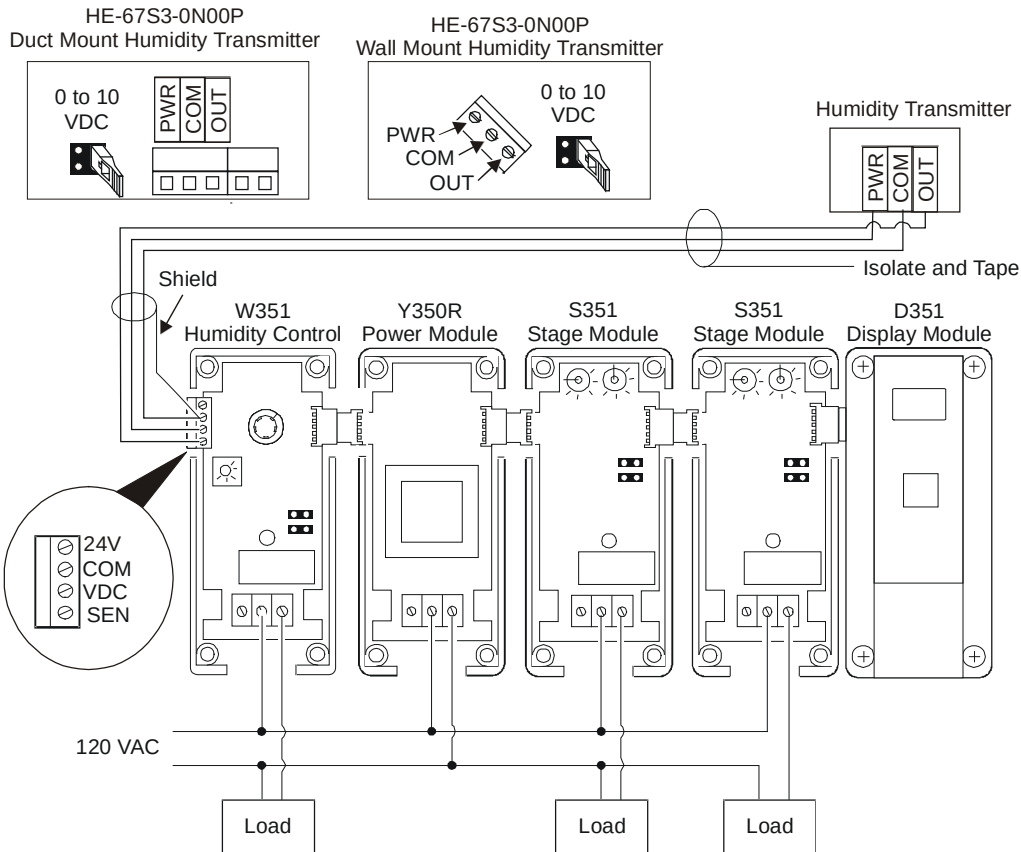
Figure 6: System 350 Modules Powered by a Y350R Power Module with the Humidity Transmitter 50-250 Feet from the W351 Control
