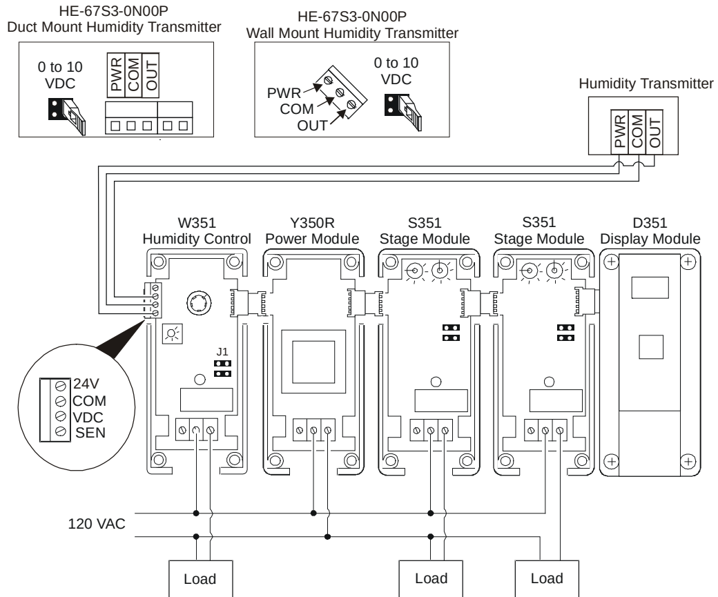
Figure 5: W351 Humidity Control (Dehumidification Mode) Powered by an External Transformer with the Humidity Transmitter Less Than 50 Feet from the W351 Control
