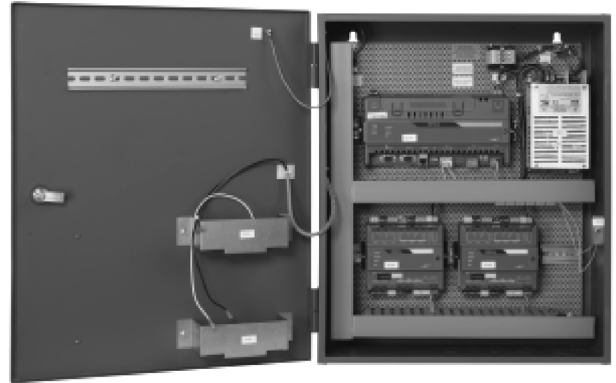
Figure 1: Security Control Panel Mounted in a 20 in. x 24 in. Enclosure
