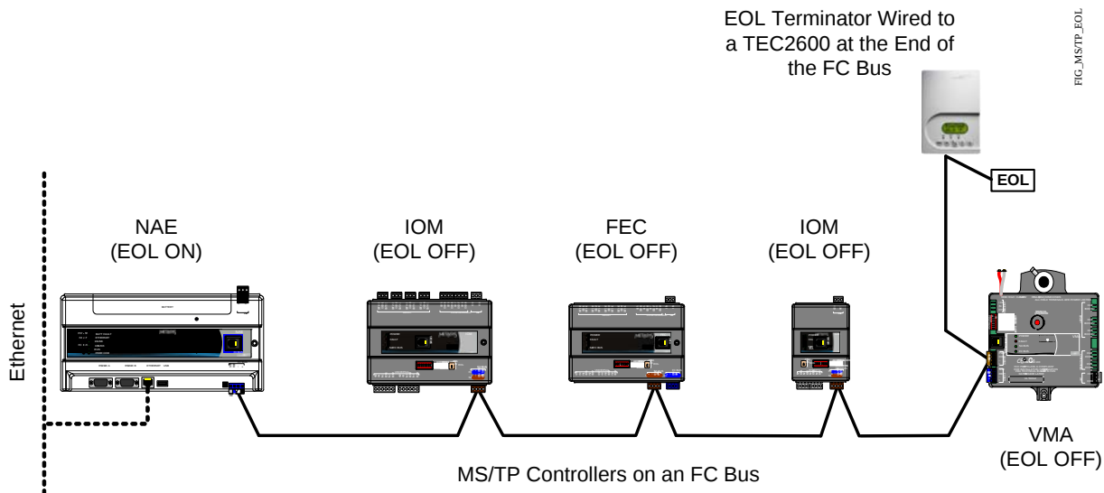
Figure 2: EOL Terminator Connected to a TEC2600 Series Thermostat to Provide End-of-Line Termination on an FC Bus
