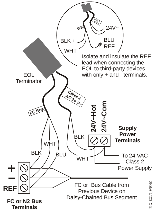
Figure 3: Wiring the EOL Terminator to a Bus-Terminating Device
