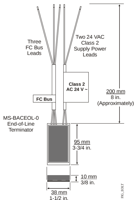
Figure 1: MS-BACEOL-0 RS485 End-of-Line Terminator Dimensions
