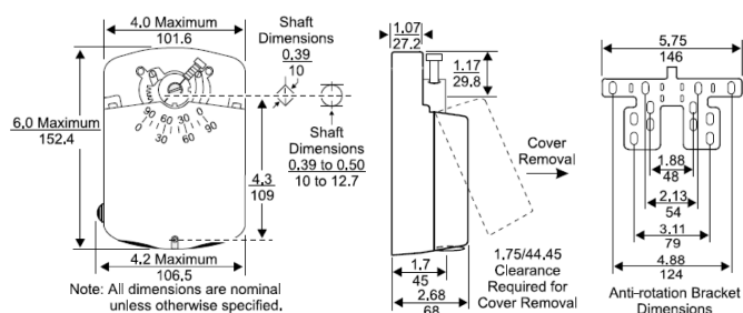
Figure 1: Dimensions, in./mm
