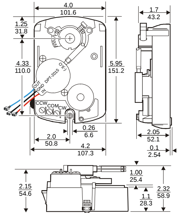
Figure 2: M9106-AGS-2N02, in. (mm)
