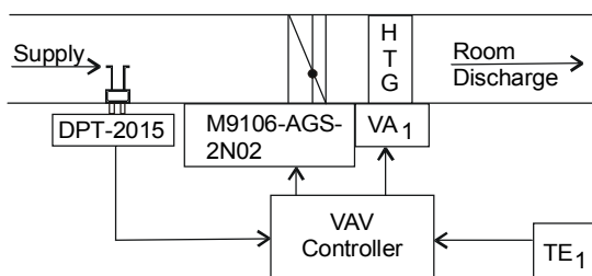
Figure 1: Single Duct, Pressure Independent
