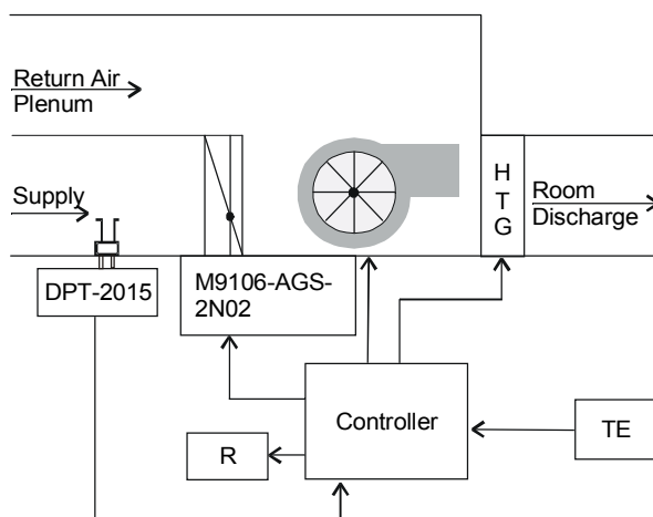
Figure 3: Single Duct, Pressure Independent with Fan Assist
