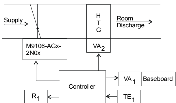
Figure 2: Single Duct, Pressure Dependent with Baseboard Heat
