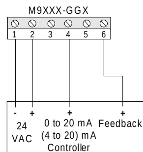
Figure 2: Using Current Controller with Feedback
