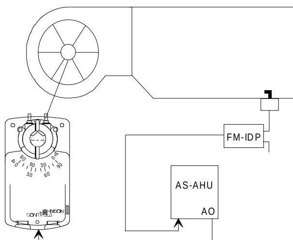
Figure 1: Inlet Vane Control
