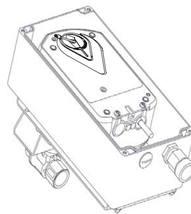
Figure 10: Actuator within M9000-341 Weather Shield Kit
