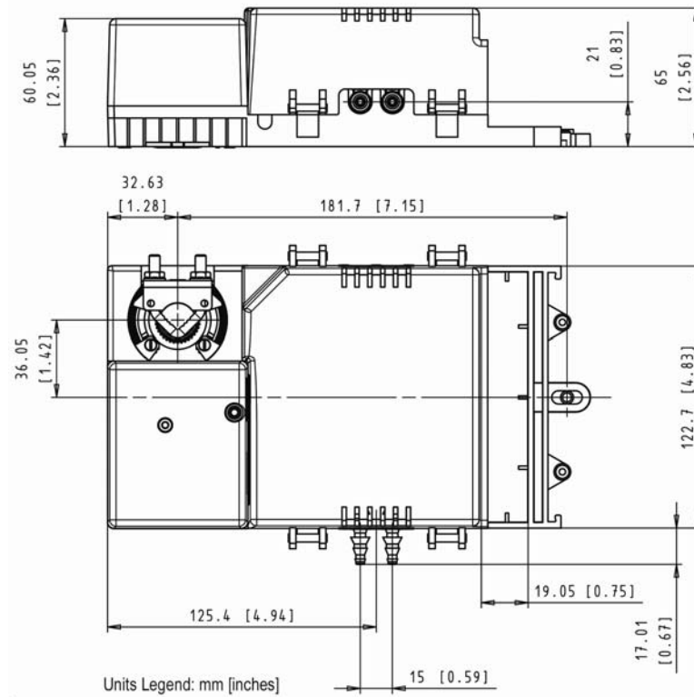
Figure 1: LN-VAVLF, LN-VAVCF, and LN-VVTLF Controller Dimensions, mm (in.)
