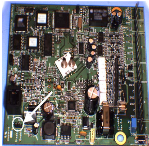
Figure 28: Enable Wireless Jumper (J16)
