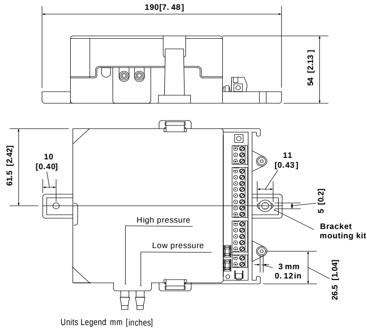
Figure 3: LN-VAVLN Controller Dimensions, mm (in.)
