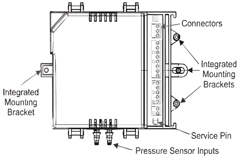
Figure 4: LN-VAVLN Controller Components
