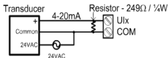
Figure 11: Current Input with Internal Power Source
