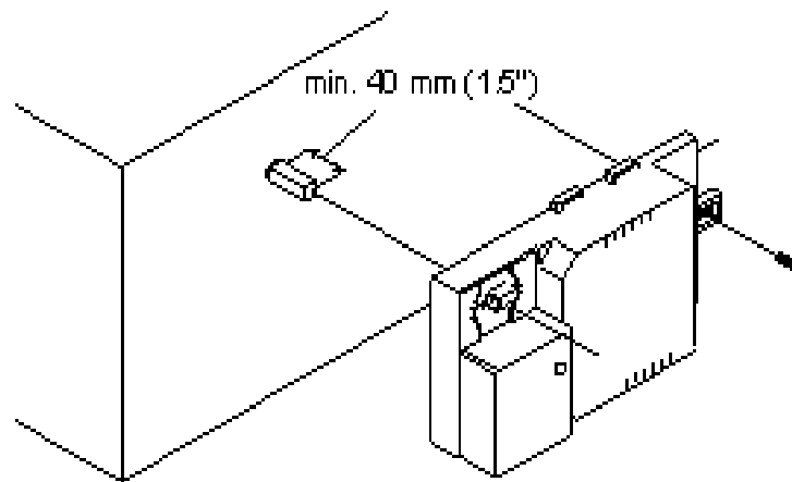
Figure 6: Mounting a VAV or VVT Device on a Damper Shaft
