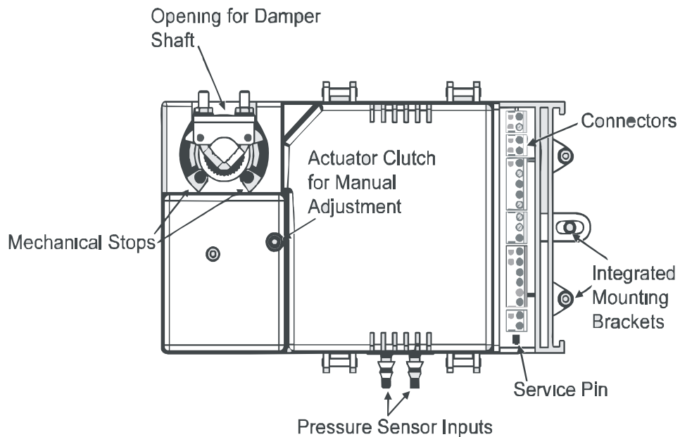
Figure 2: LN-VAVLF, LN-VVTLF, and LN-VAVCF Controller Components
