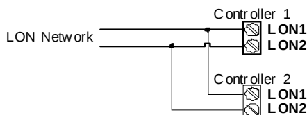
Figure 24: Communications Wiring
