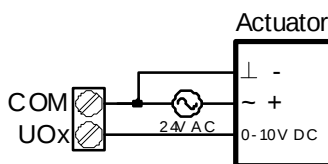
Figure 23: Voltage 0 to 10 VDC Universal Output - Analog Actuator
