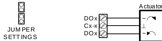
Figure 19: Digital Output with Internal Power Supply - Floating Actuator
