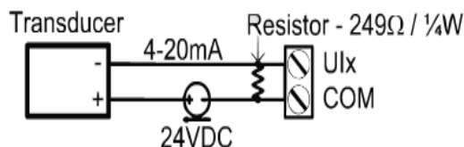
Figure 10: Current Input - 2 Wire Transducer
