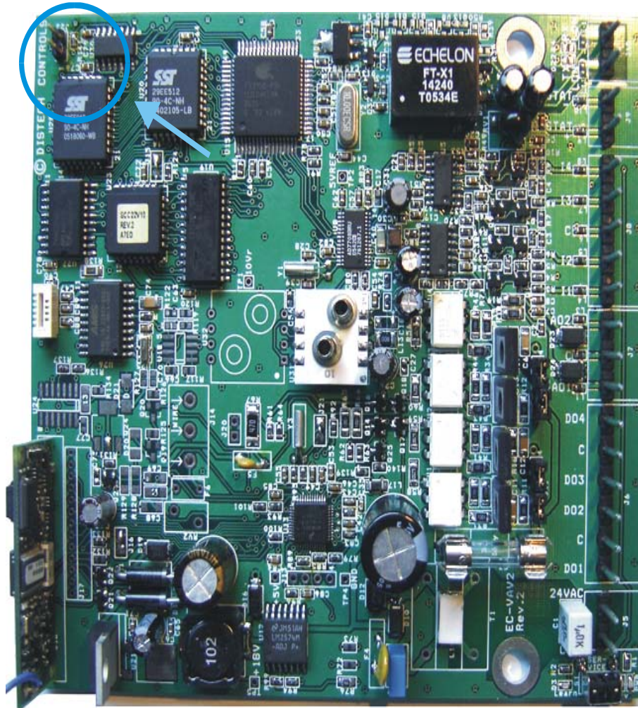
Figure 25: E-Blank Jumper (J22) Location
