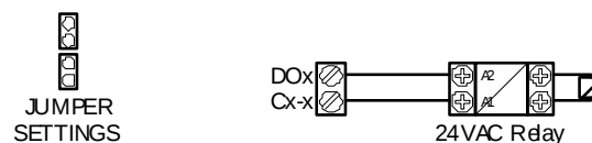
Figure 17: Digital Output with Internal Power Supply
