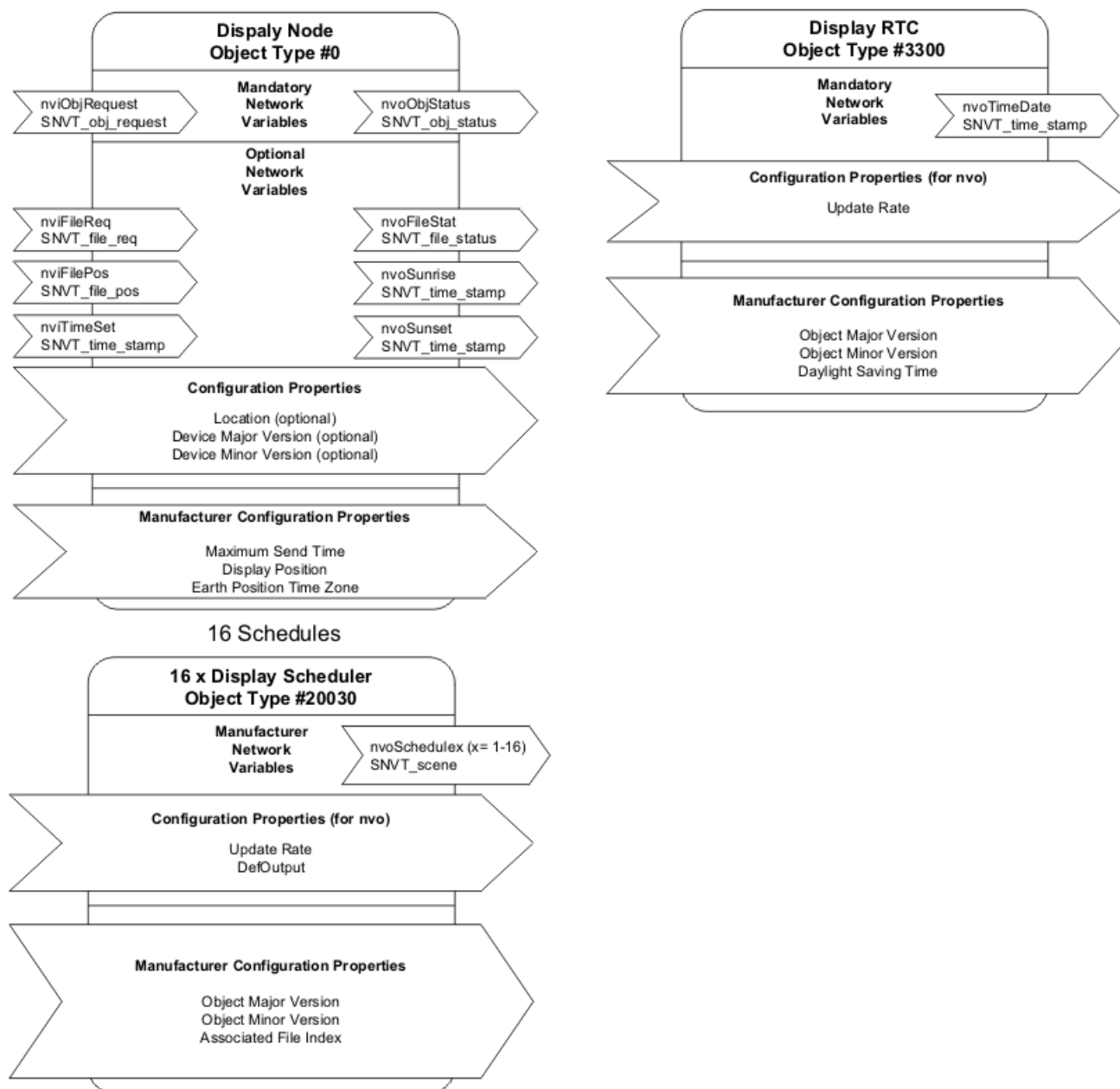
Figure 4: LONMARK Objects and Network Variables – LN-DSWSCx-0
