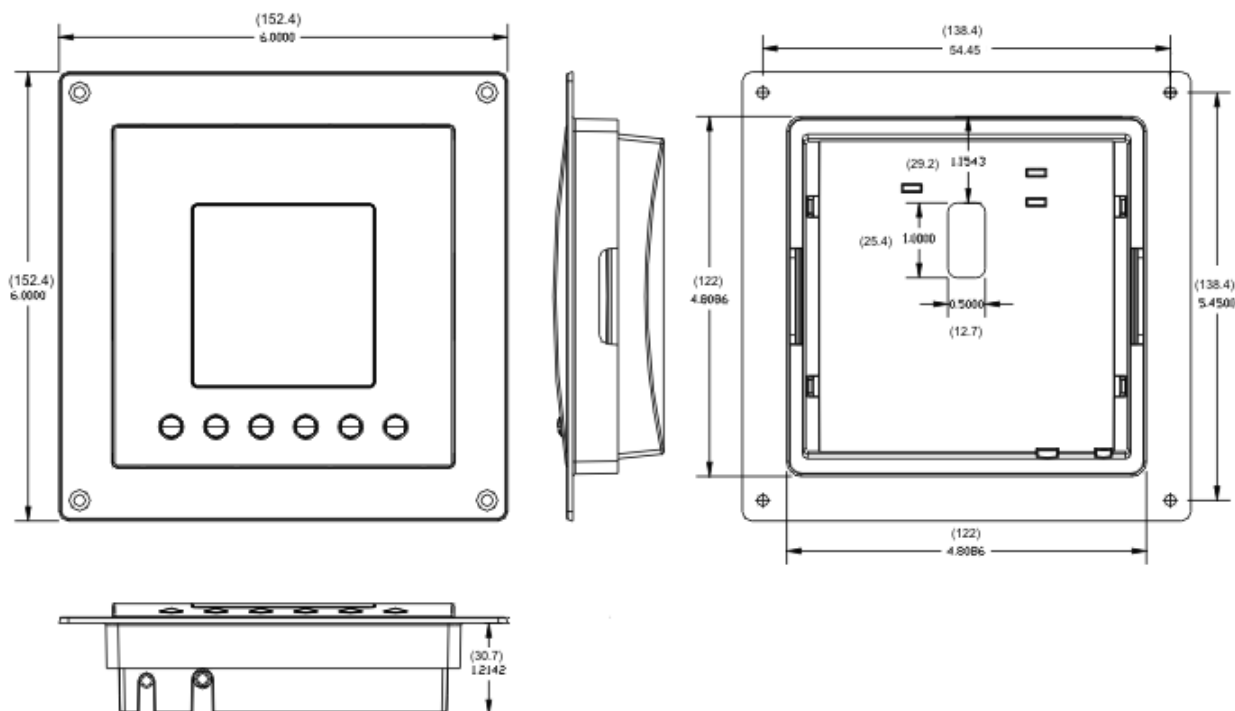
Figure 2: LN Series Display Flush Mount Dimensions, in. (mm)
