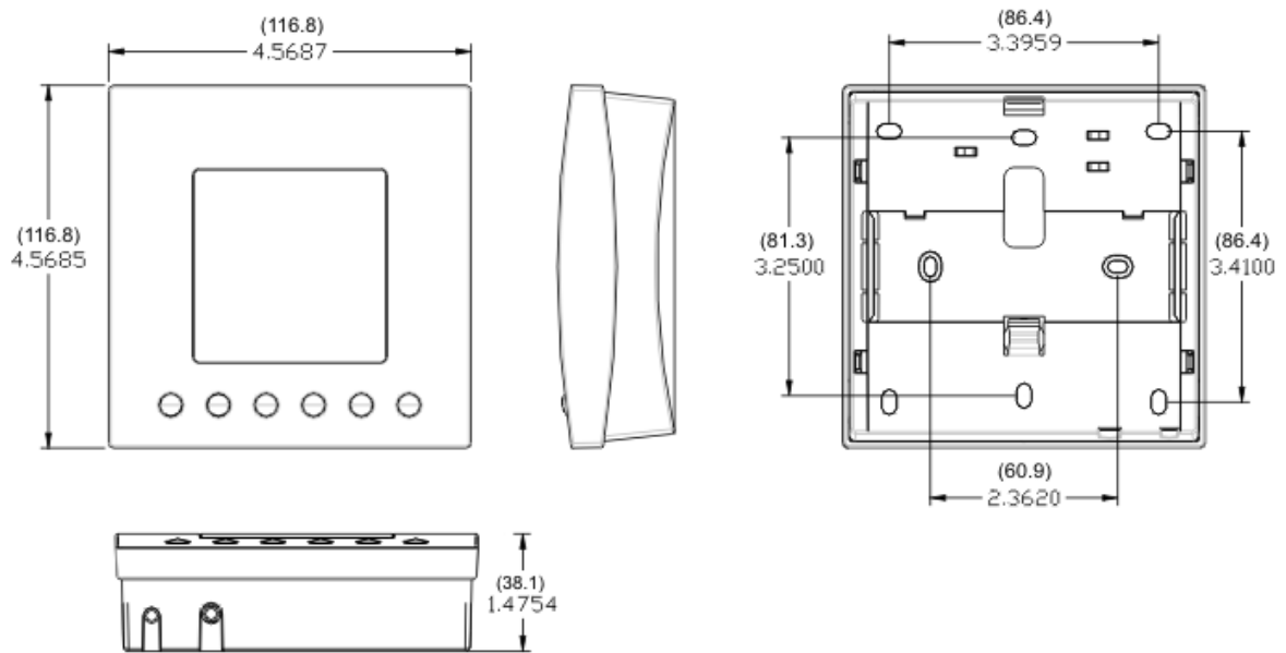
Figure 3: LN Series Display (Surface Mount) Dimensions, in. (mm)
