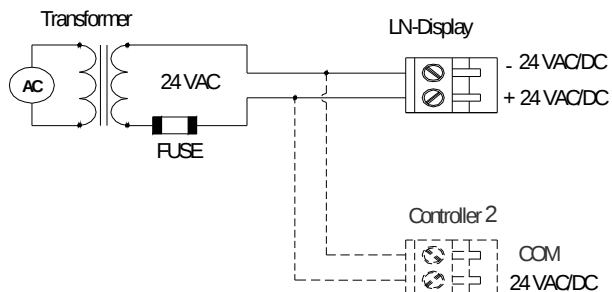
Figure 10: Power Wiring
