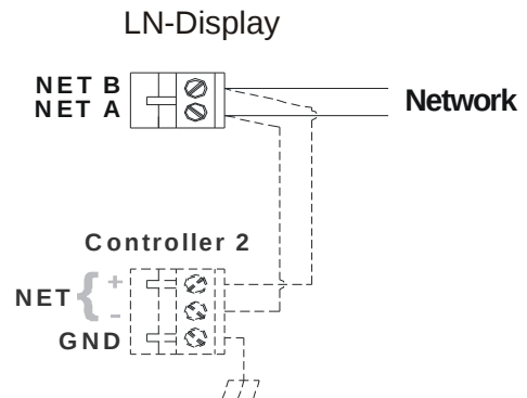
Figure 11: Communications Wiring
