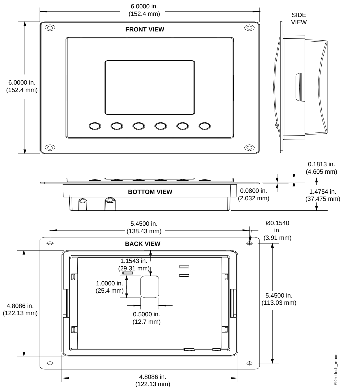
Figure 2: Flush-Mount Casing Dimensions
