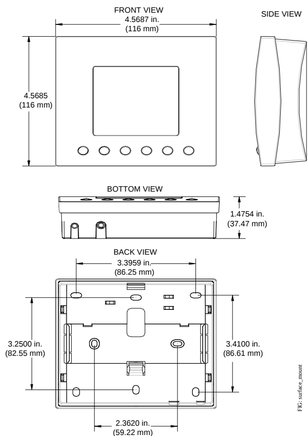
Figure 1: Surface Mount Casing Dimensions, in. (mm)
