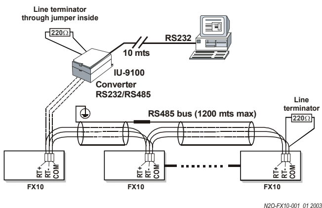
Figure 3: Network lay-out
