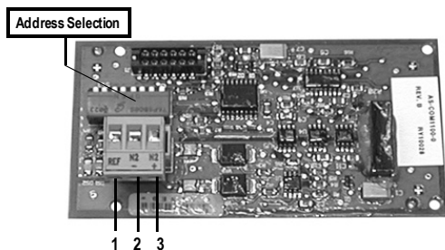
Figure 1: N2Open Serial Card
