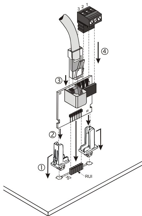
DLI Insertion and Connection
