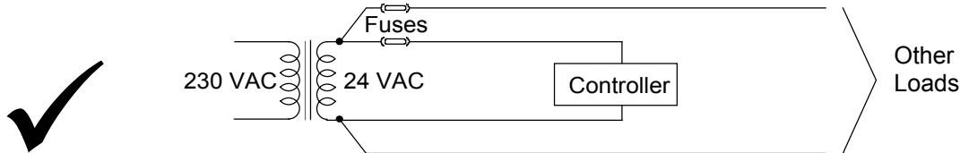
Correct Wiring of Controller to 24 V Transformer
