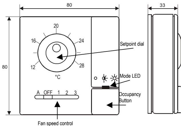
Figure 2: Dimensions (mm)
