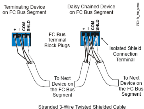
Figure 4: FC Bus Terminal Block Wiring
