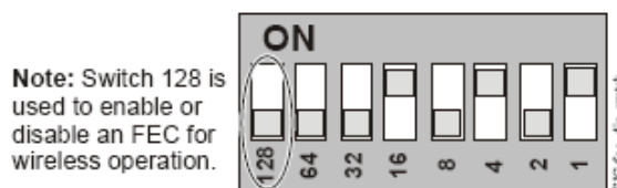
Figure 9: Device Address Switches Set to 21
