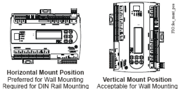
Figure 1: Controller Mounting Positions
