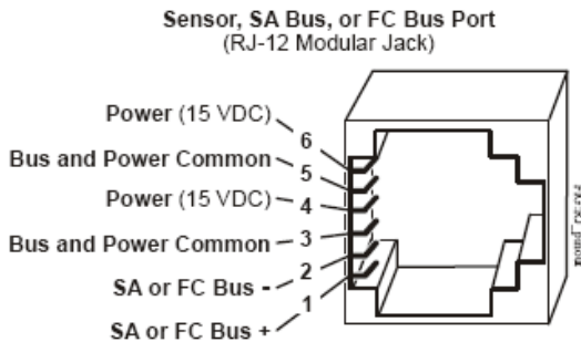
Figure 6: Pin Number Assignments for Sensor, SA Bus, and FC Bus Ports on FEC, IOM, and VMA16
