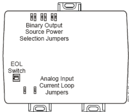
Figure 10: FEC16 with Cover Removed Showing Jumper and EOL Switch Positions
