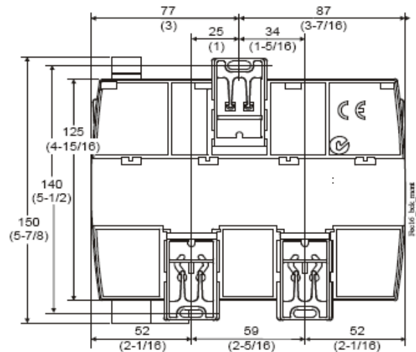
Figure 2: Back of FEC16 Controller Showing Extended Mounting Clips, DIN Rail Channel, and
