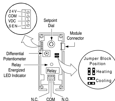
Interior of A350A/B
