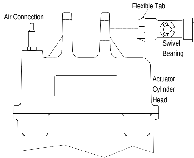
Figure 1: Installing Swivel Bearing
