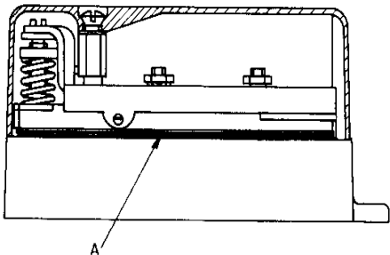
Fig. 4: C-9506 Air Switching Cumulator
