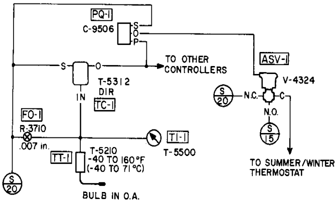
Fig. 3: Typical Application using C-9506
