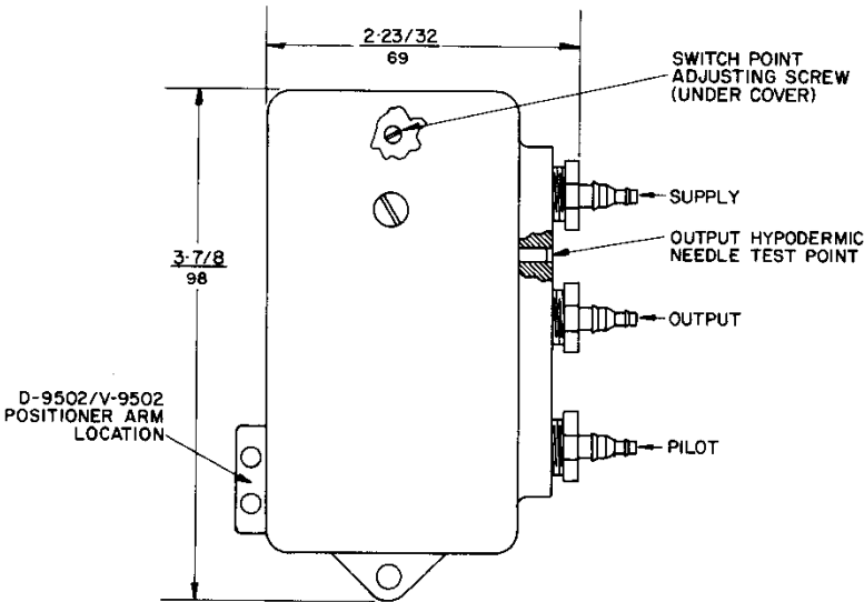
Fig. 2: C-9506 Dimensions in. mm
