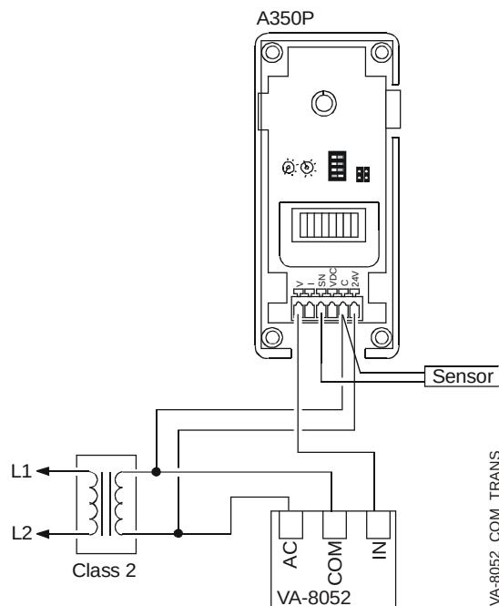
Figure 2: Wiring an A350P Controller to a VA-8052 Valve Actuator Using a Common Transformer to Power the Application
