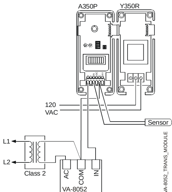
Figure 4: Wiring an A350P Controller and Y350R Power Module to a VA-8052 Valve Actuator with a Separate Power Supply Transformer
