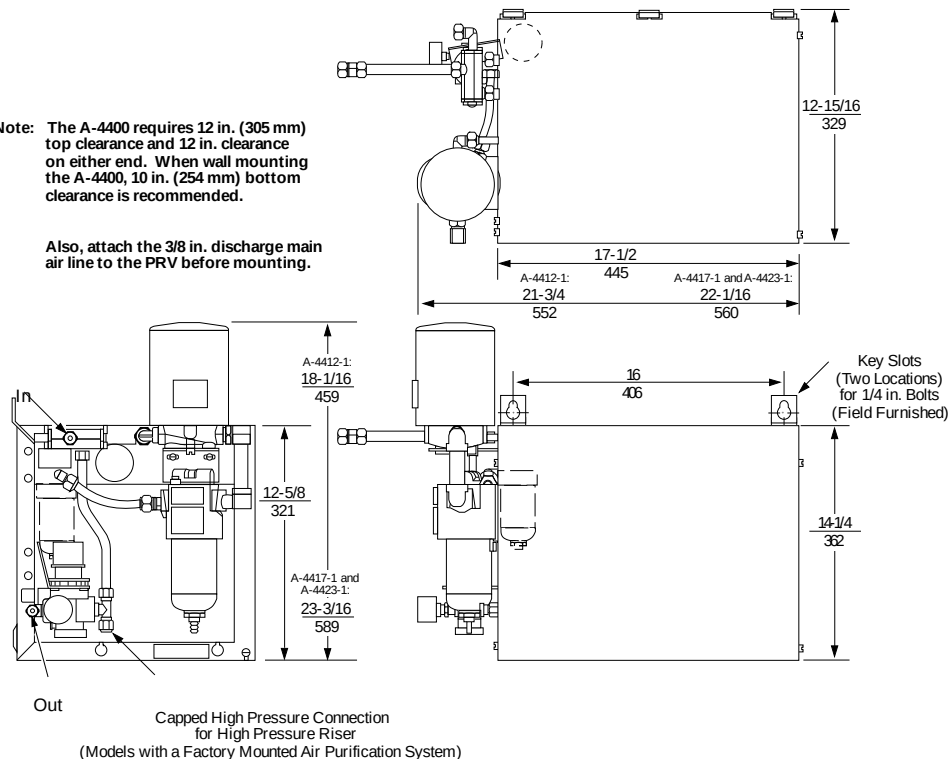
Figure 1: A-4400 Series Refrigerated Air Dryer Shown with Optional Factory Mounted Air Purification System
