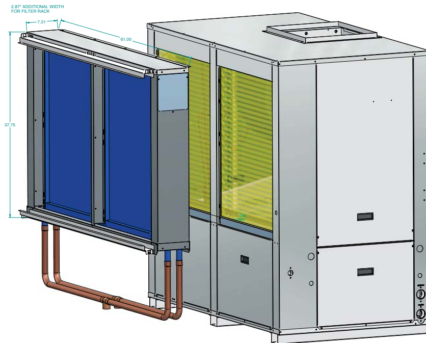
RL080-120 ECONOMIZER OPTION (RIGHT RETURN SHOWN)
