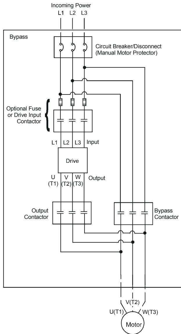
Figure 5: IntelliPass Power and Motor Terminal Wiring Example
