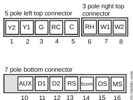
Figure 5: Terminal Blocks
