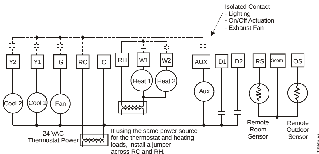
Figure 6: Wiring the T600MSx-3 Thermostats
