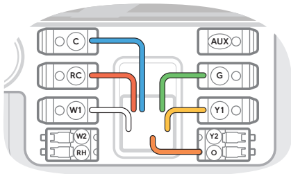
Furnace
