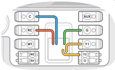
Air Handler
