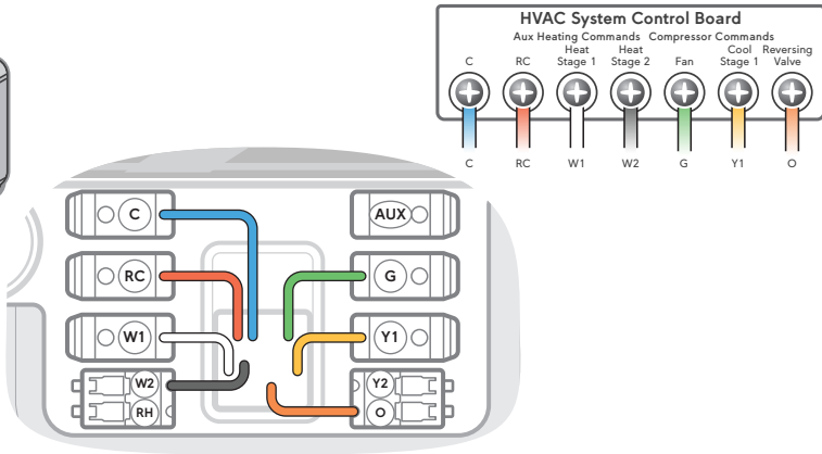
Heat Pump
