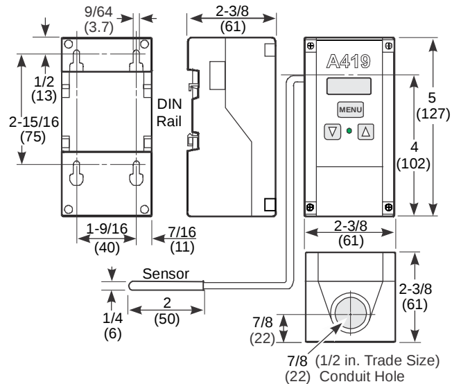
Figure 1: Dimensions for A419 Temperature Controls with NEMA 1 Enclosures, in./(mm)
